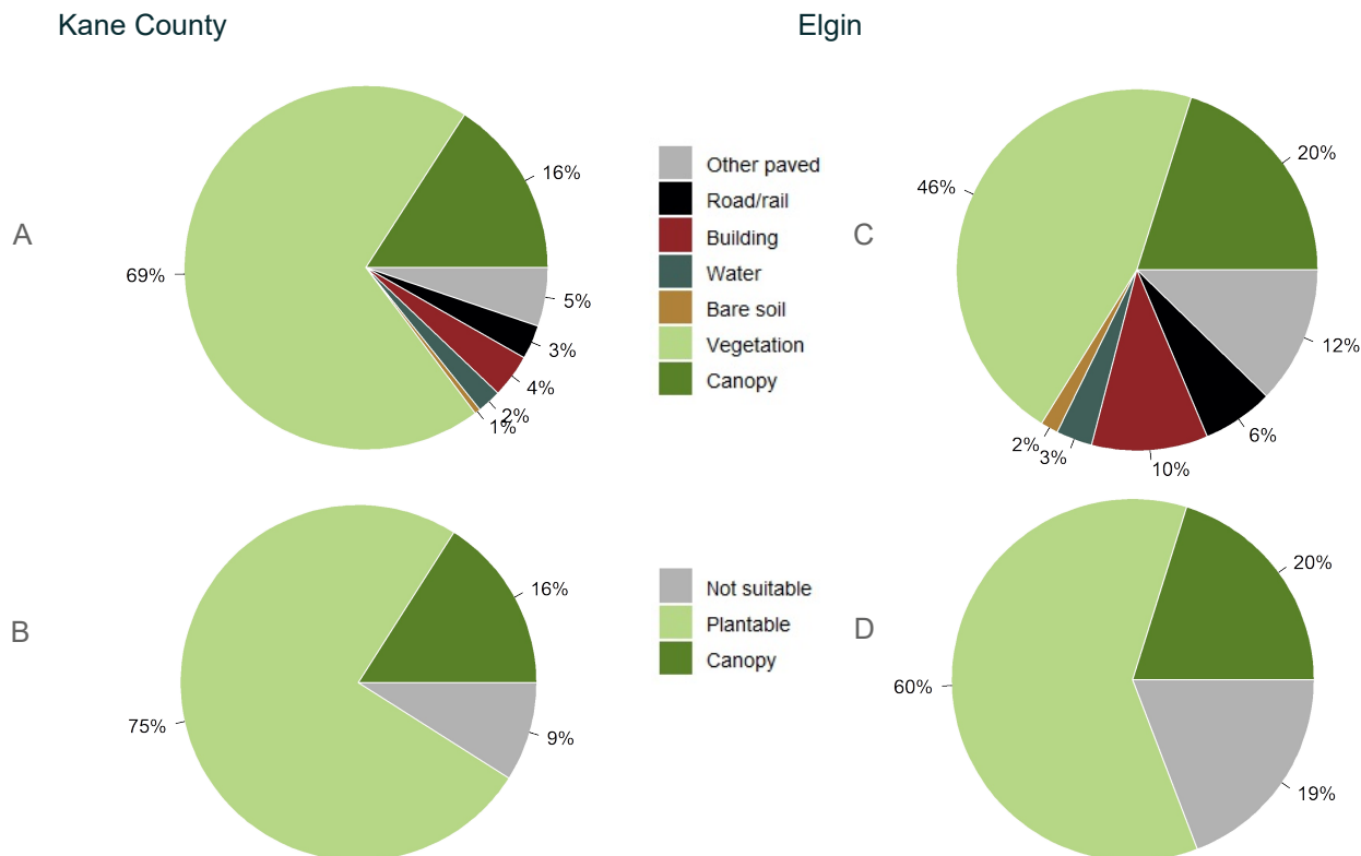
Figure 2: Land cover distribution and plantable space in Kane County (A and B), and in Elgin (C and D).
