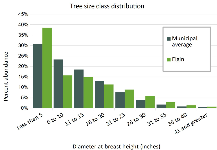
Figure 13: Distribution of tree sizes in Elgin and across all municipal inventories.
