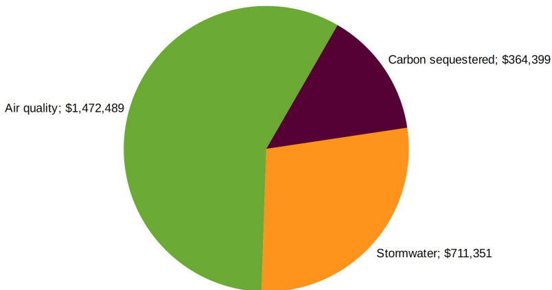
Figure 14: Trees offer myriad benefits, including intercepting stormwater, improving air quality and removing carbon from the atmosphere.
