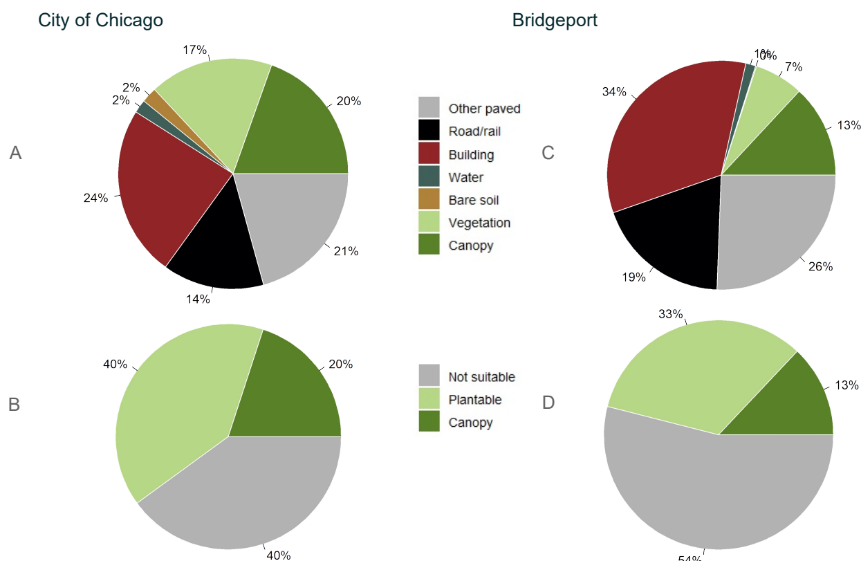
Figure 2: Land cover distribution and plantable space in the City of Chicago (A and B) and in Bridgeport (C and D).
