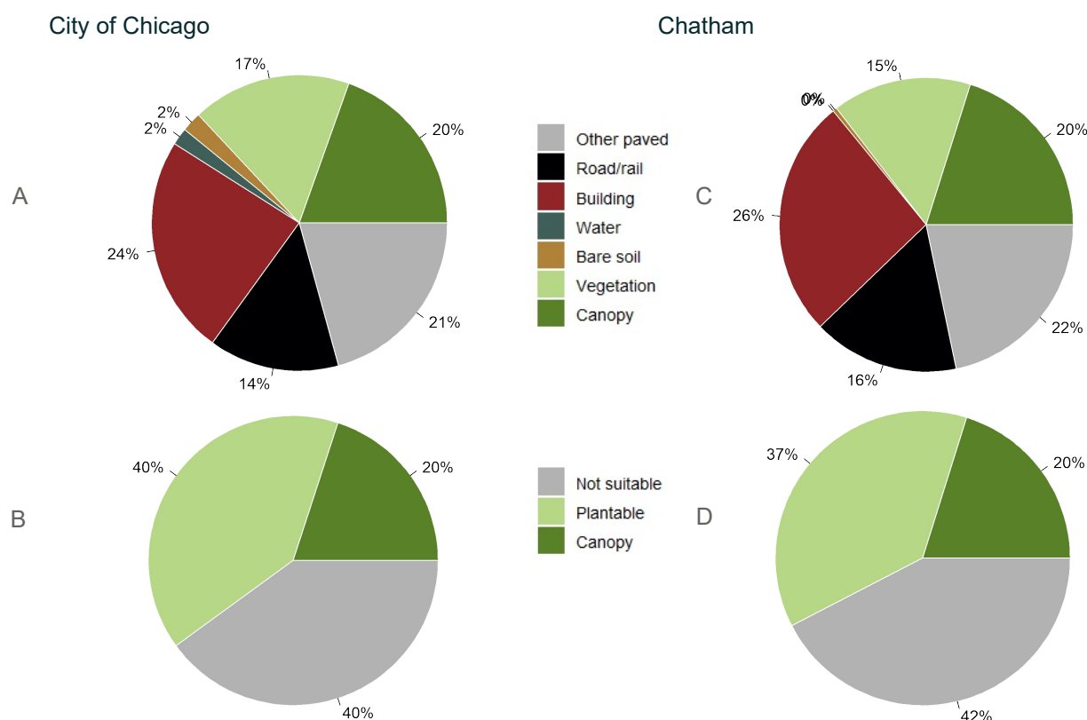
Figure 2: Land cover distribution and plantable space in the City of Chicago (A and B) and in Chatham (C and D).
