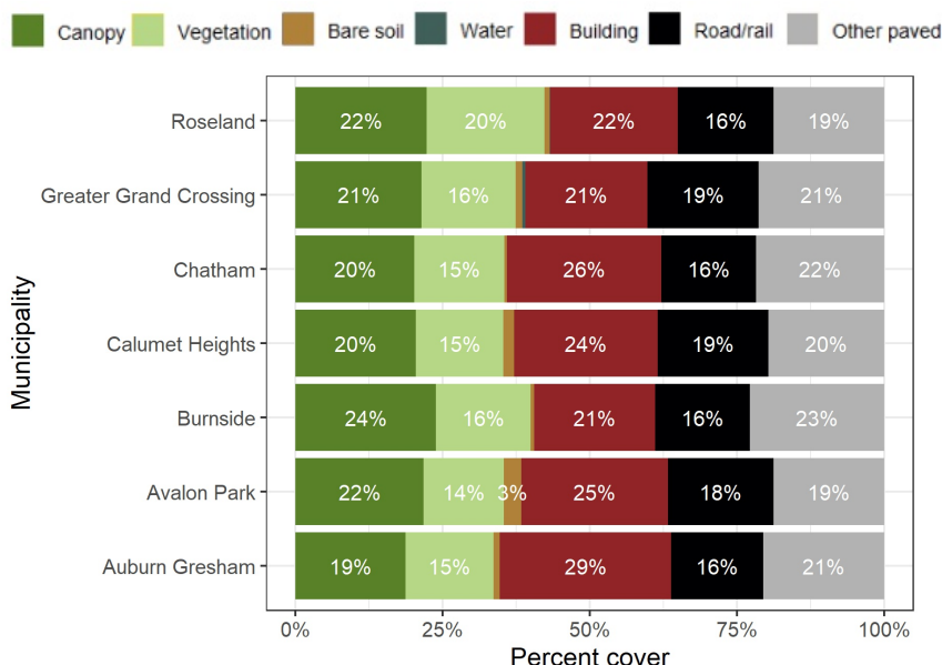
Figure 7: Comparison of land cover of Chatham and its neighbors.
