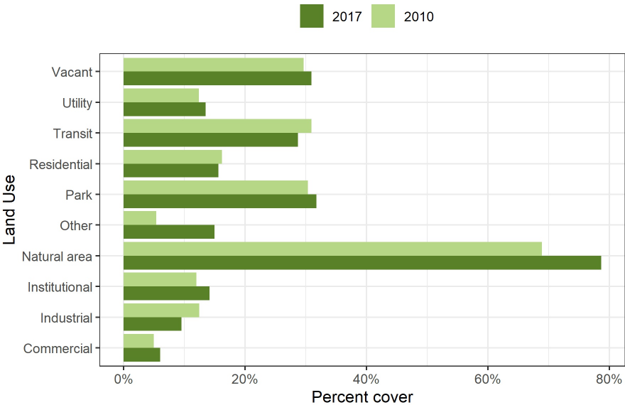
Figure 9: Canopy change across land use types in Chatham.
