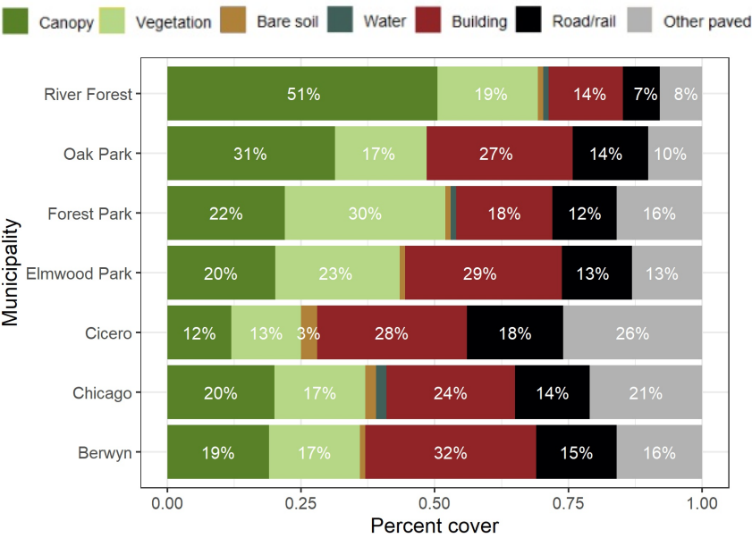
Figure 7: Comparison of land cover of Oak Park and its neighbors.
