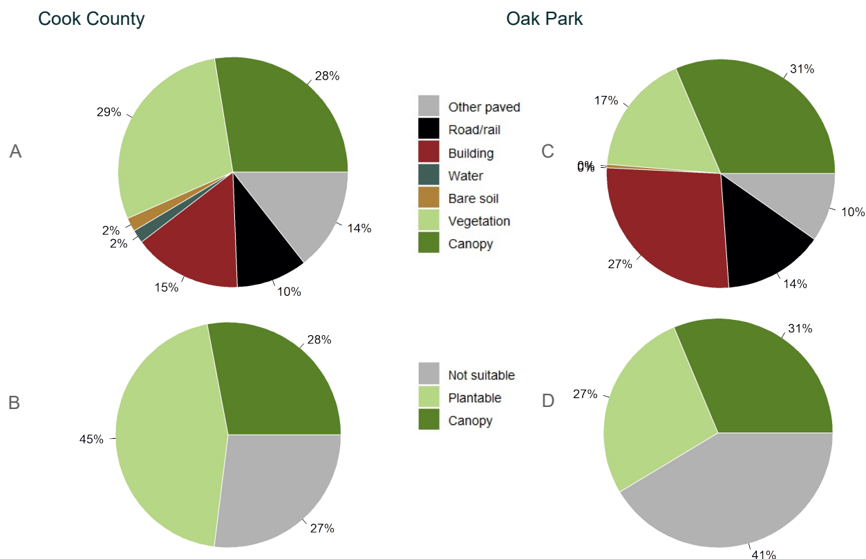
Figure 2: Land cover distribution and plantable space in Cook County (A and B) and in Oak Park (C and D).
