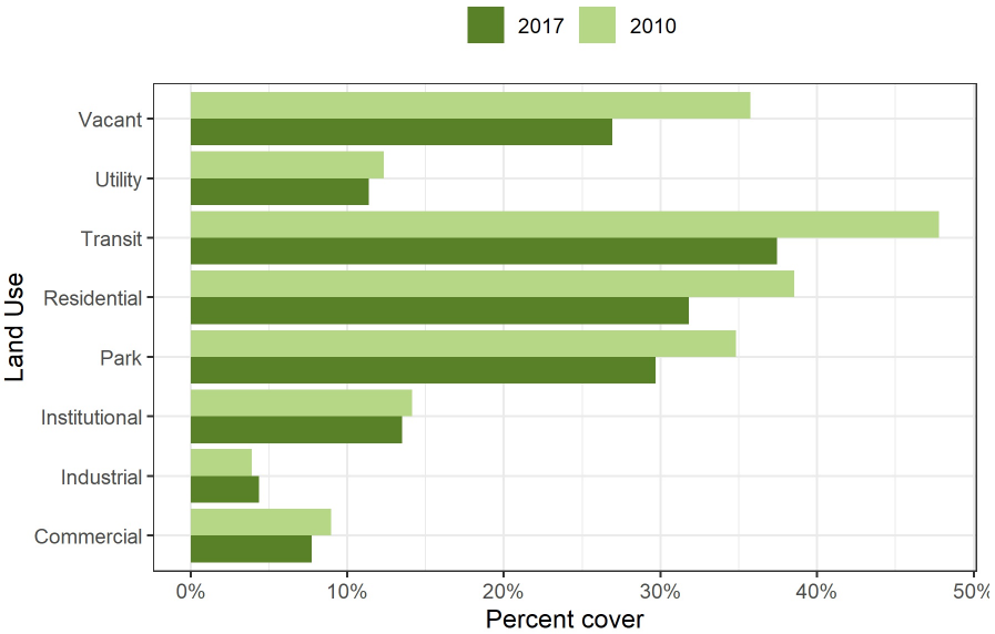
Figure 9: Canopy change across land use types in Oak Park.
