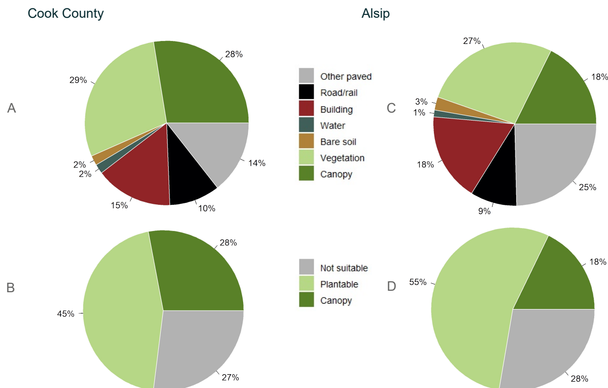
Figure 2: Land cover distribution and plantable space in Cook County (A and B), and in Alsip (C and D).
