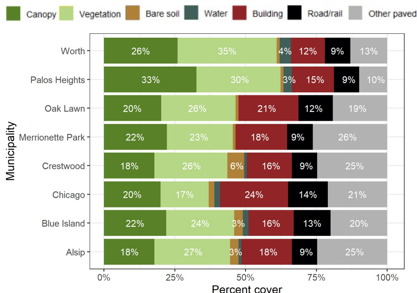
Figure 7: Comparison of land cover of Alsip and its neighbors.
