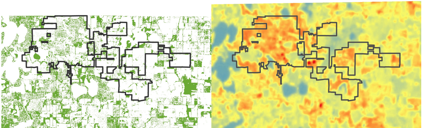
Figure 13: The image on the left shows tree canopy and on the right shows surface temperature. Surface temperature was calculated using a LandSat8 image from July 2017. Areas that have higher tree canopy tend to have lower temperatures.
