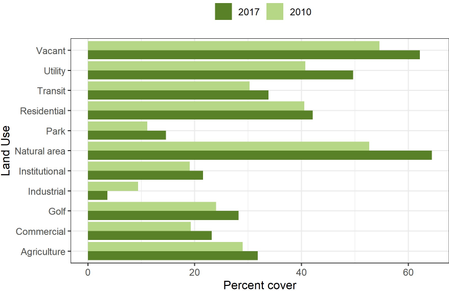
Figure 9: Canopy change across land use types in Beach Park.
