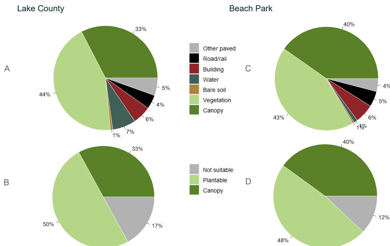
Figure 2: Land cover distribution and plantable space in Lake County (A and B), and in Beach Park (C and D).
