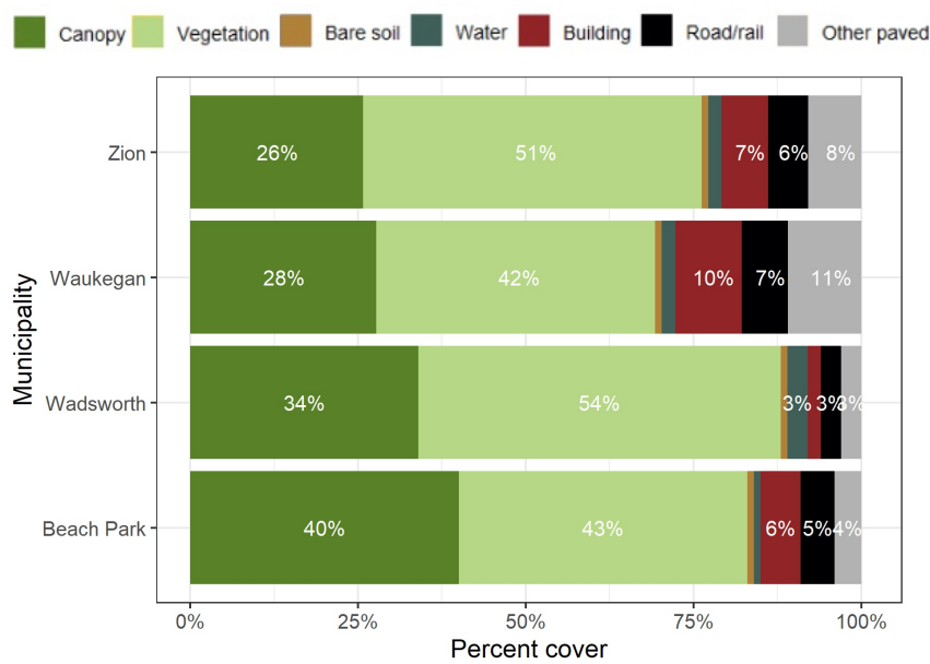
Figure 7: Comparison of land cover of Beach Park and its neighbors.
