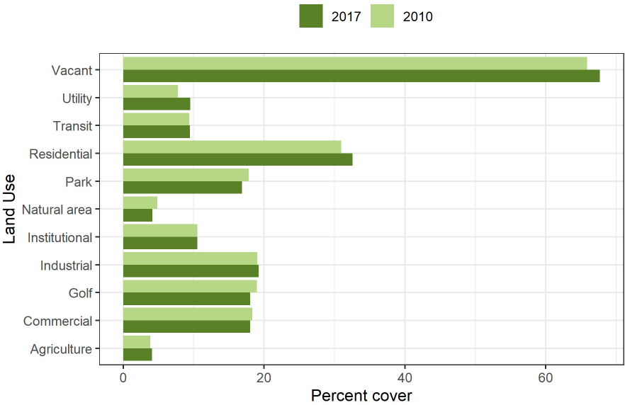
Figure 9: Canopy change across land use types in Burlington.
