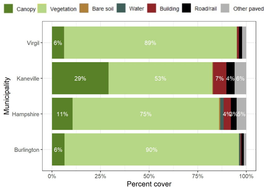
Figure 7: Comparison of land cover of Burlington and its neighbors.
