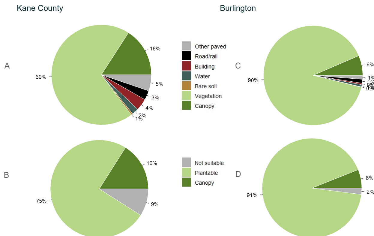
Figure 2: Land cover distribution and plantable space in Kane County (A and B), and in Burlington (C and D).
