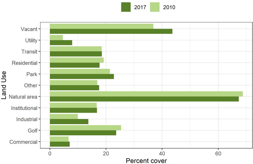
Figure 9: Canopy change across land use types in Calumet City.
