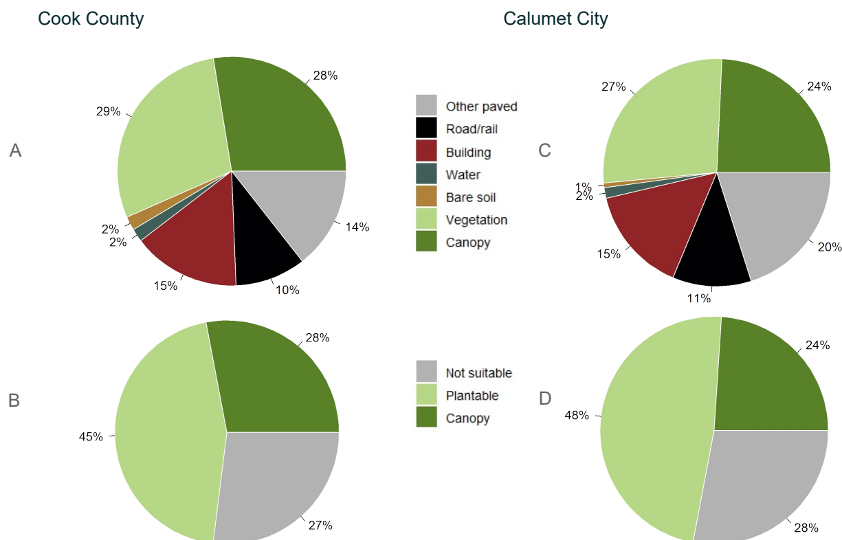
Figure 2: Land cover distribution and plantable space in Cook County (A and B), and in Calumet City (C and D).
