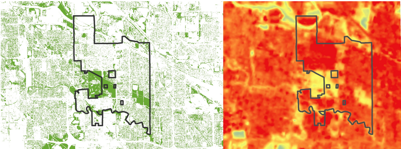
Figure 13: The image on the left shows tree canopy and on the right shows surface temperature. Surface temperature was calculated using a LandSat8 image from July 2017. Areas that have higher tree canopy tend to have lower temperatures.
