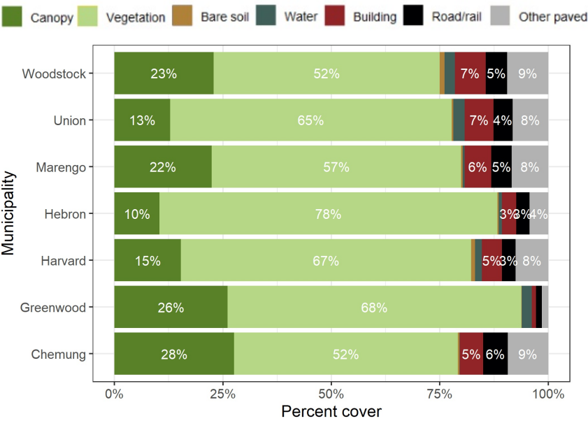
Figure 7: Comparison of land cover of Chemung and its neighbors.
