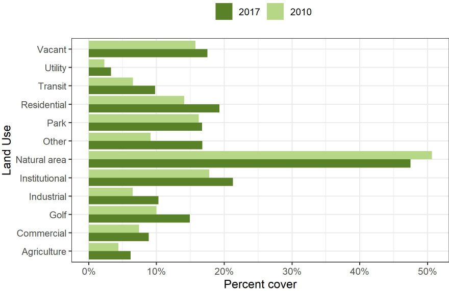
Figure 9: Canopy change across land use types in Elburn.
