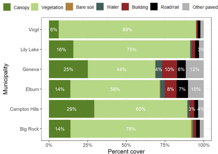
Figure 7: Comparison of land cover of Elburn and its neighbors.
