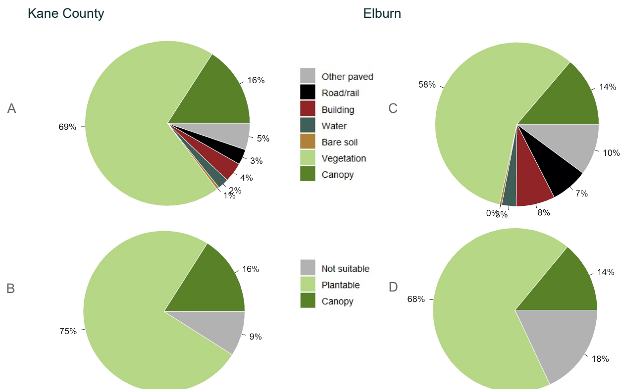
Figure 2: Land cover distribution and plantable space in Kane County (A and B), and in Elburn (C and D).
