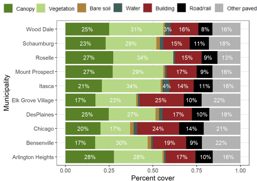
Figure 7: Comparison of land cover of Elk Grove Village and its neighbors.
