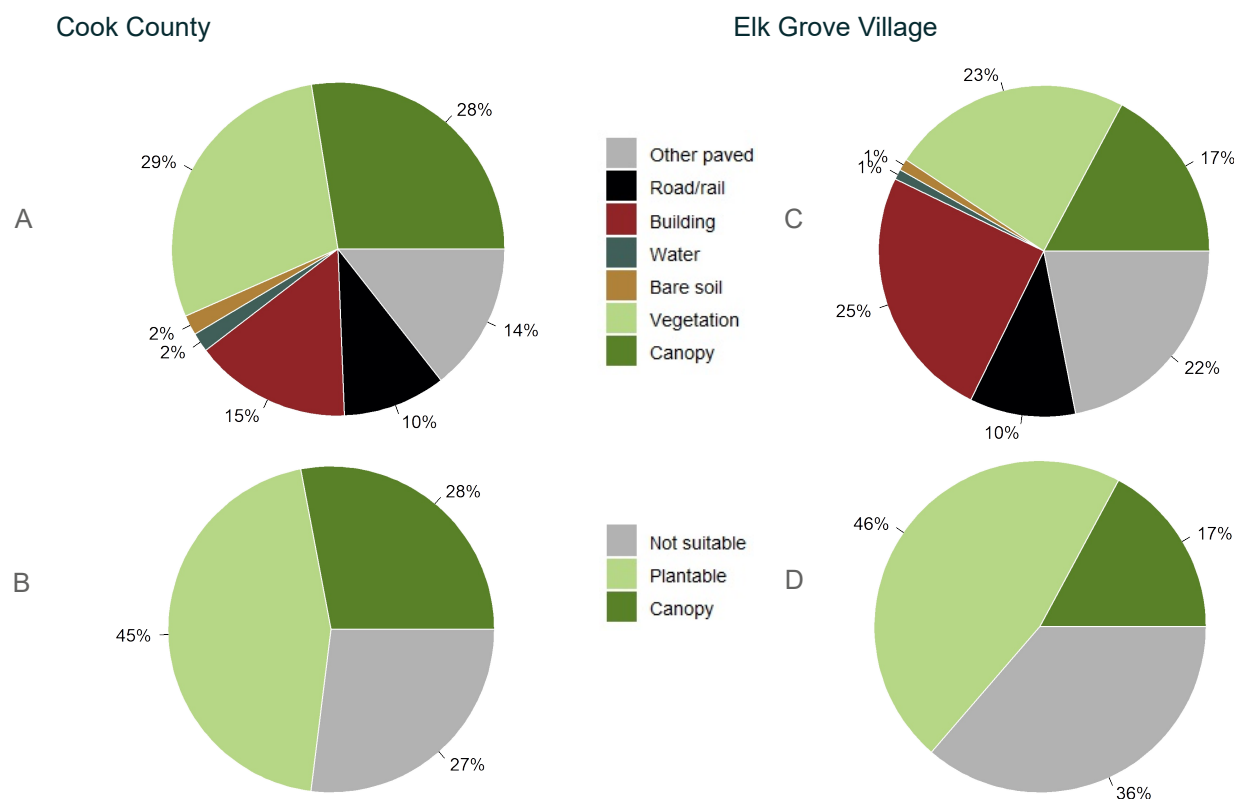
Figure 2: Land cover distribution and plantable space in Cook County (A and B), and in Elk Grove Village (C and D).
