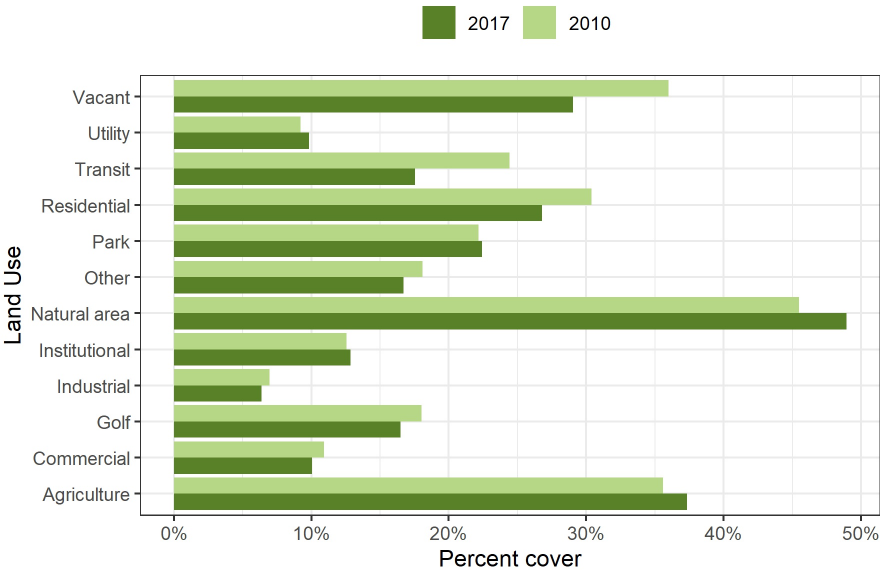
Figure 9: Canopy change across land use types in Elk Grove Village.
