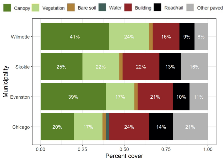
Figure 7: Comparison of land cover of Evanston and its neighbors.
