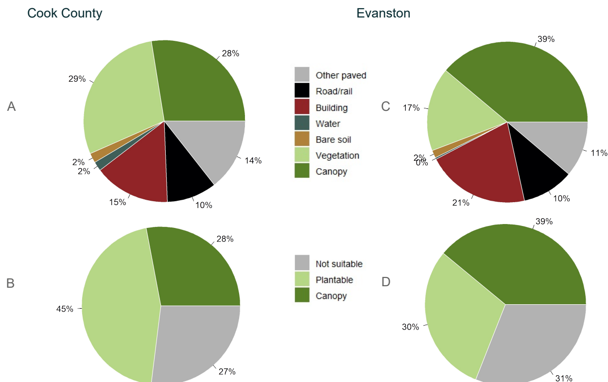
Figure 2: Land cover distribution and plantable space in Cook County (A and B), and in Evanston (C and D).
