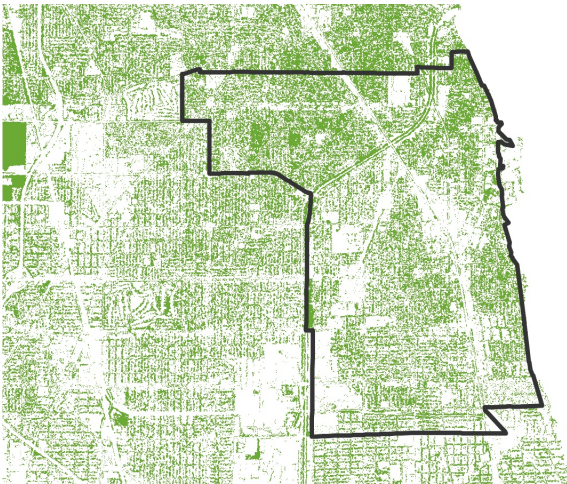
Figure 15: The image on the left shows tree canopy and on the right shows surface temperature. Surface temperature was calculated using a LandSat8 image from July 2017. Areas that have higher tree canopy tend to have lower temperatures.
