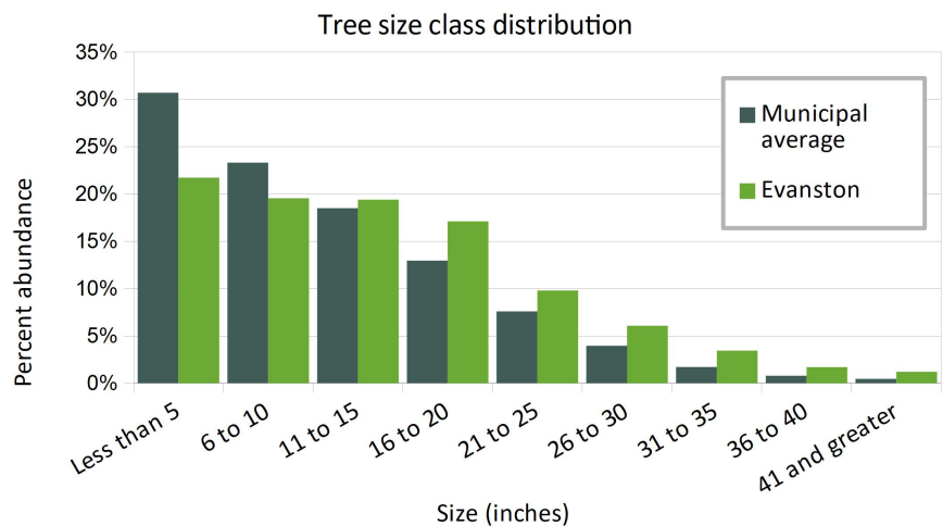
Figure 13: Distribution of tree sizes in Evanston and across all municipal inventories.
