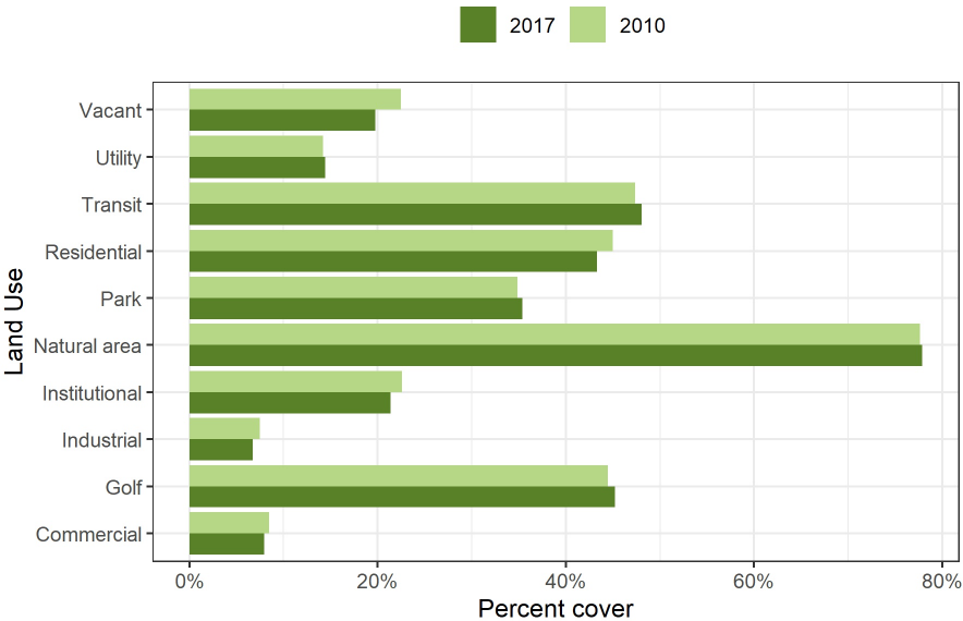
Figure 9: Canopy change across land use types in Evanston.
