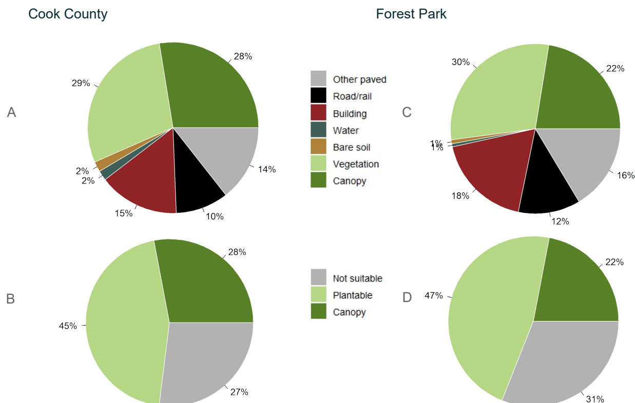
Figure 2: Land cover distribution and plantable space in Cook County (A and B), and in Forest Park (C and D).
