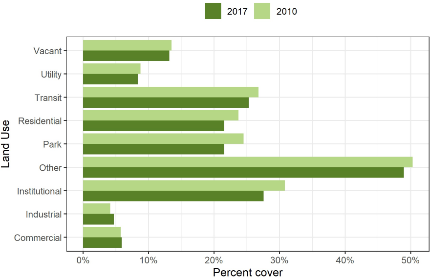
Figure 9: Canopy change across land use types in Forest Park.
