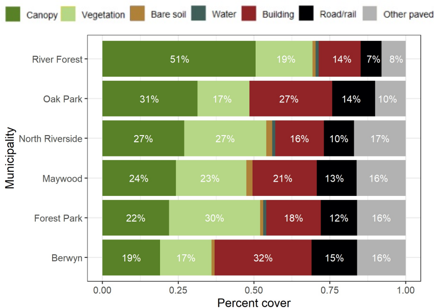
Figure 7: Comparison of land cover of Forest Park and its neighbors.
