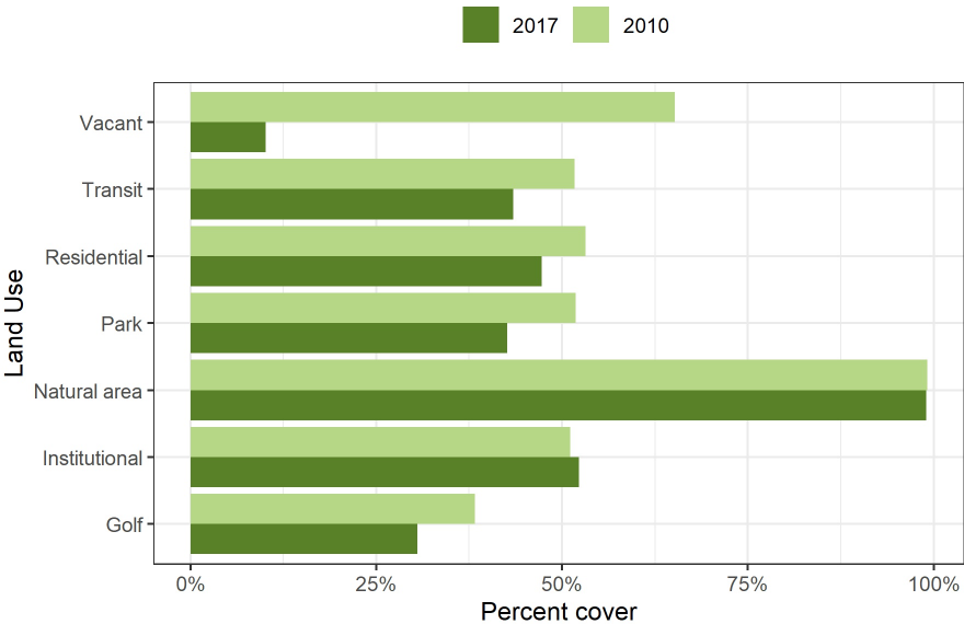
Figure 9: Canopy change across land use types in Golf.
