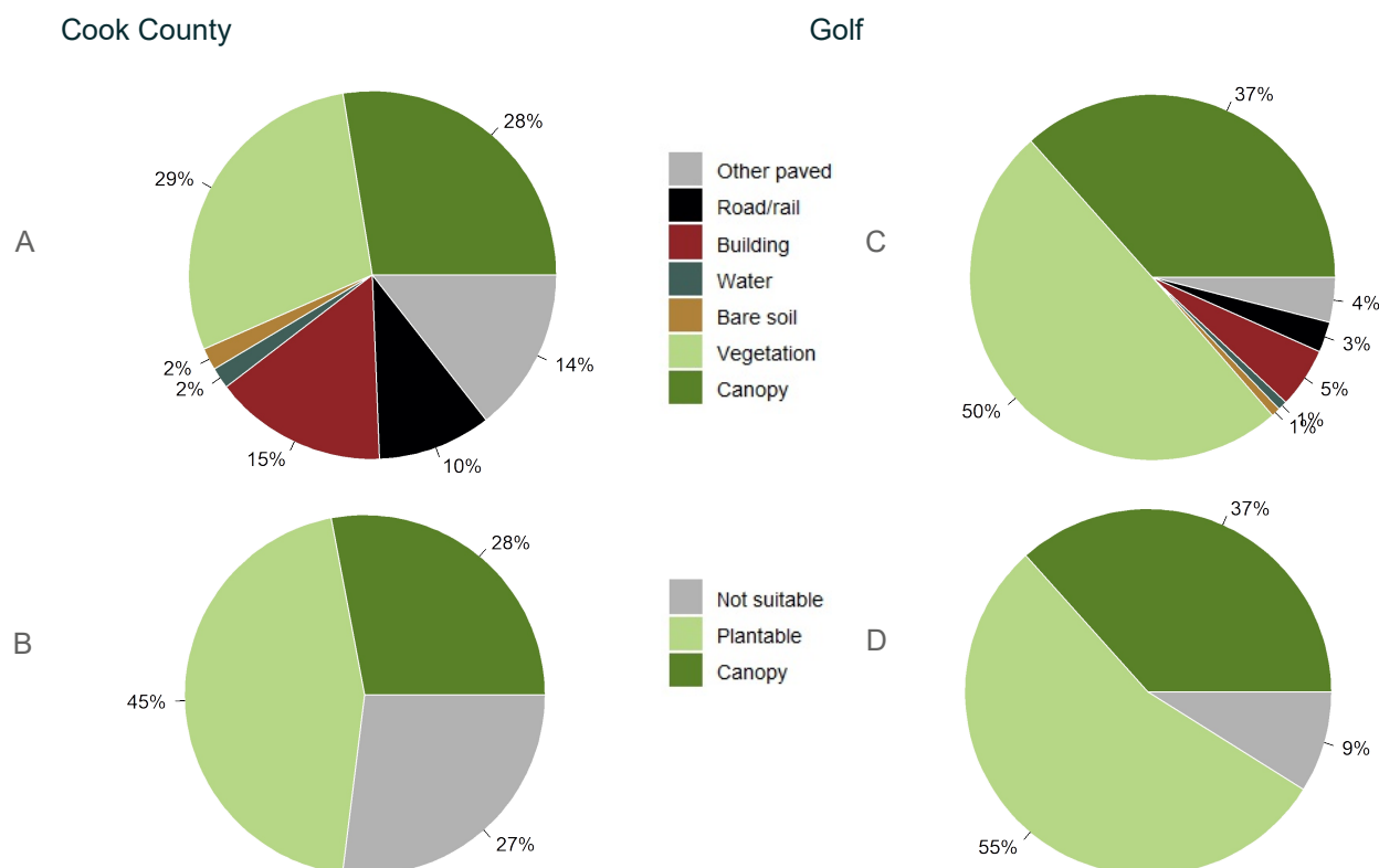
Figure 2: Land cover distribution and plantable space in Cook County (A and B), and in Golf (C and D).
