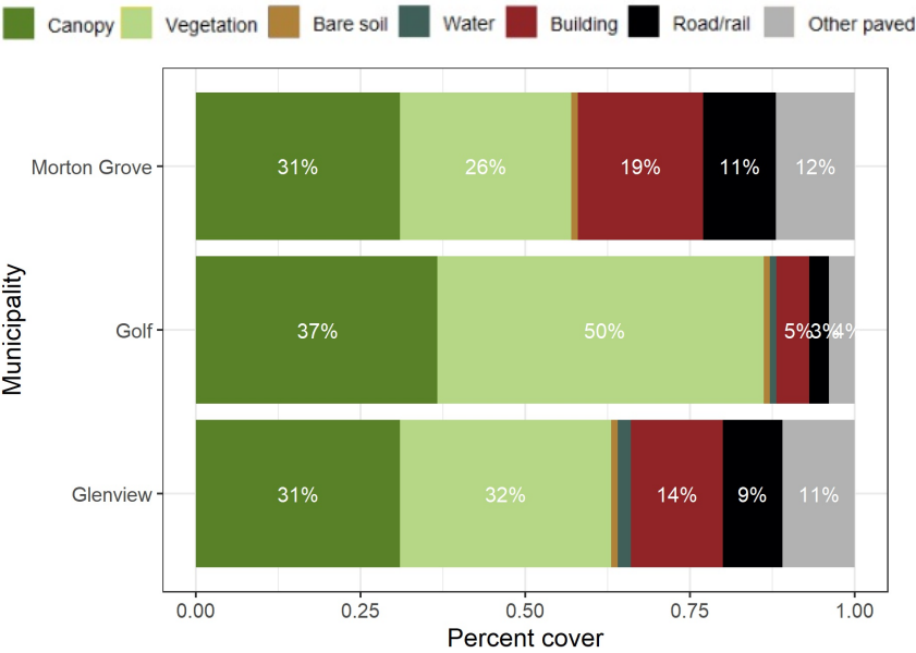
Figure 7: Comparison of land cover of Golf and its neighbors.
