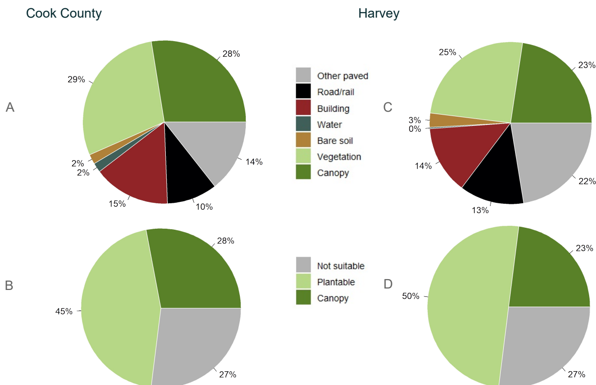
Figure 2: Land cover distribution and plantable space in Cook County (A and B), and in Harvey (C and D).
