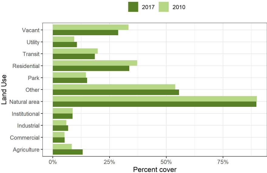
Figure 9: Canopy change across land use types in Harvey.
