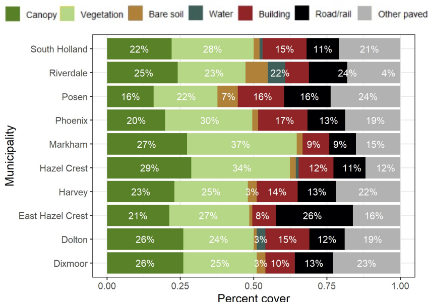
Figure 7: Comparison of land cover of Harvey and its neighbors.
