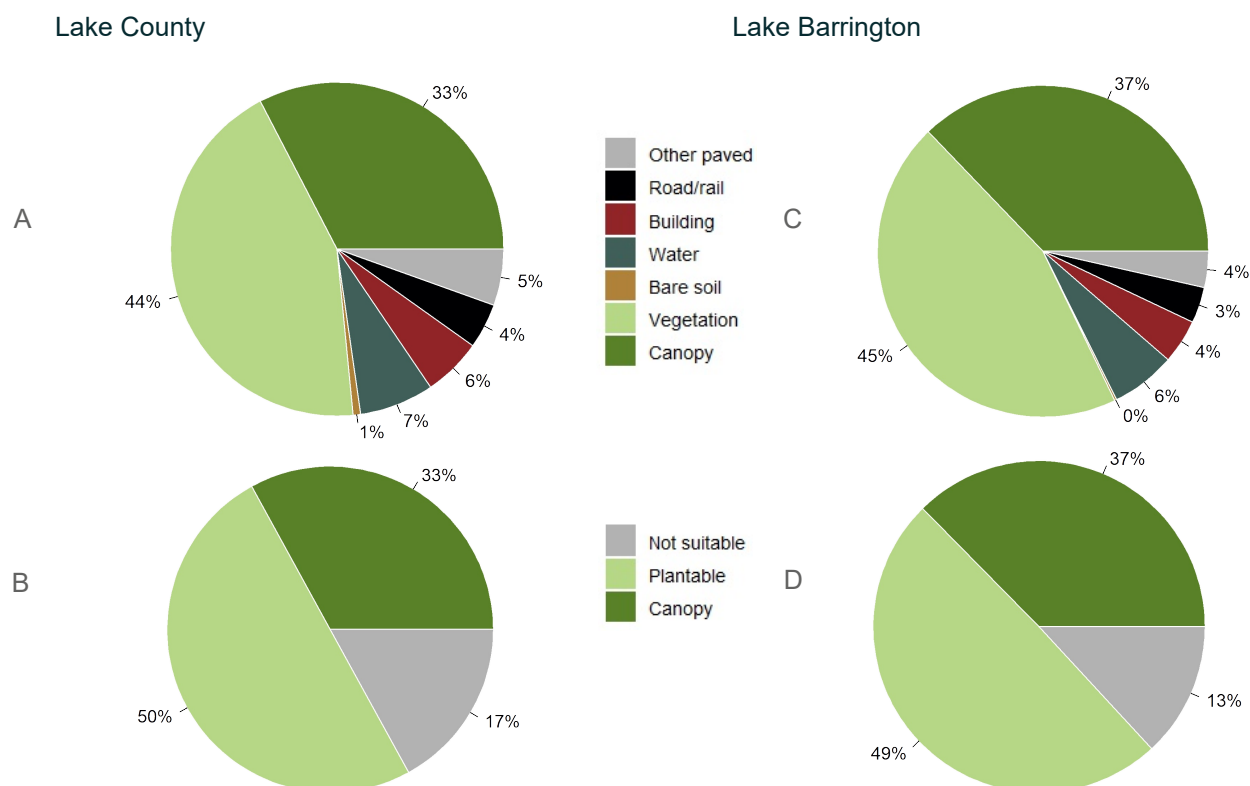
Figure 2: Land cover distribution and plantable space in Lake County (A and B), and in Lake Barrington (C and D).
