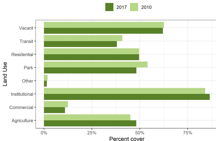
Figure 9: Canopy change across land use types in Lake Catherine.
