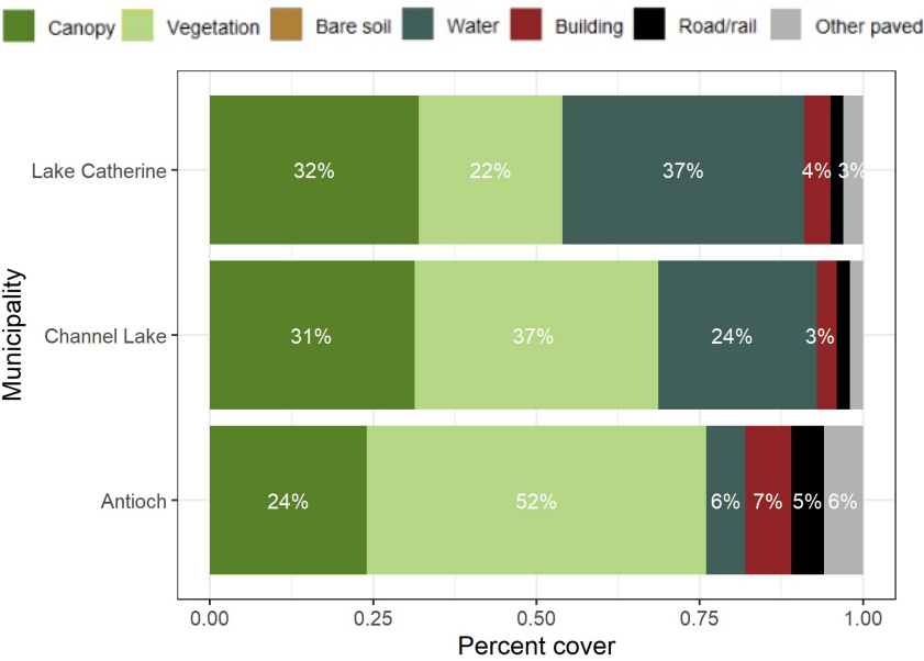
Figure 7: Comparison of land cover of Lake Catherine and its neighbors.
