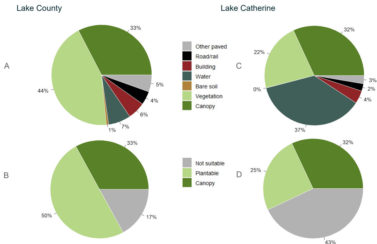
Figure 2: Land cover distribution and plantable space in Lake County (A and B), and in Lake Catherine (C and D).
