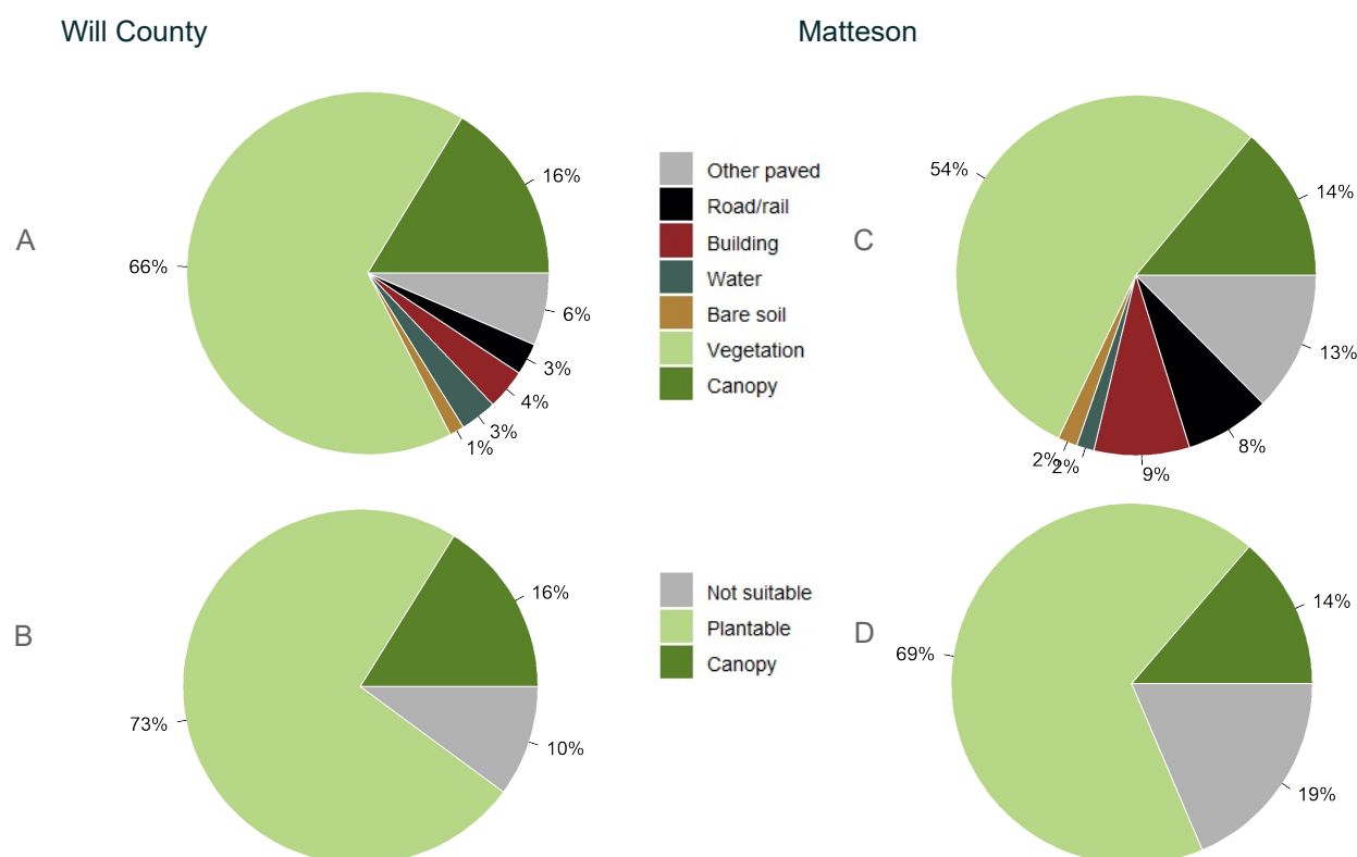
Figure 2: Land cover distribution and plantable space in Will County (A and B) and in Matteson (C and D).
