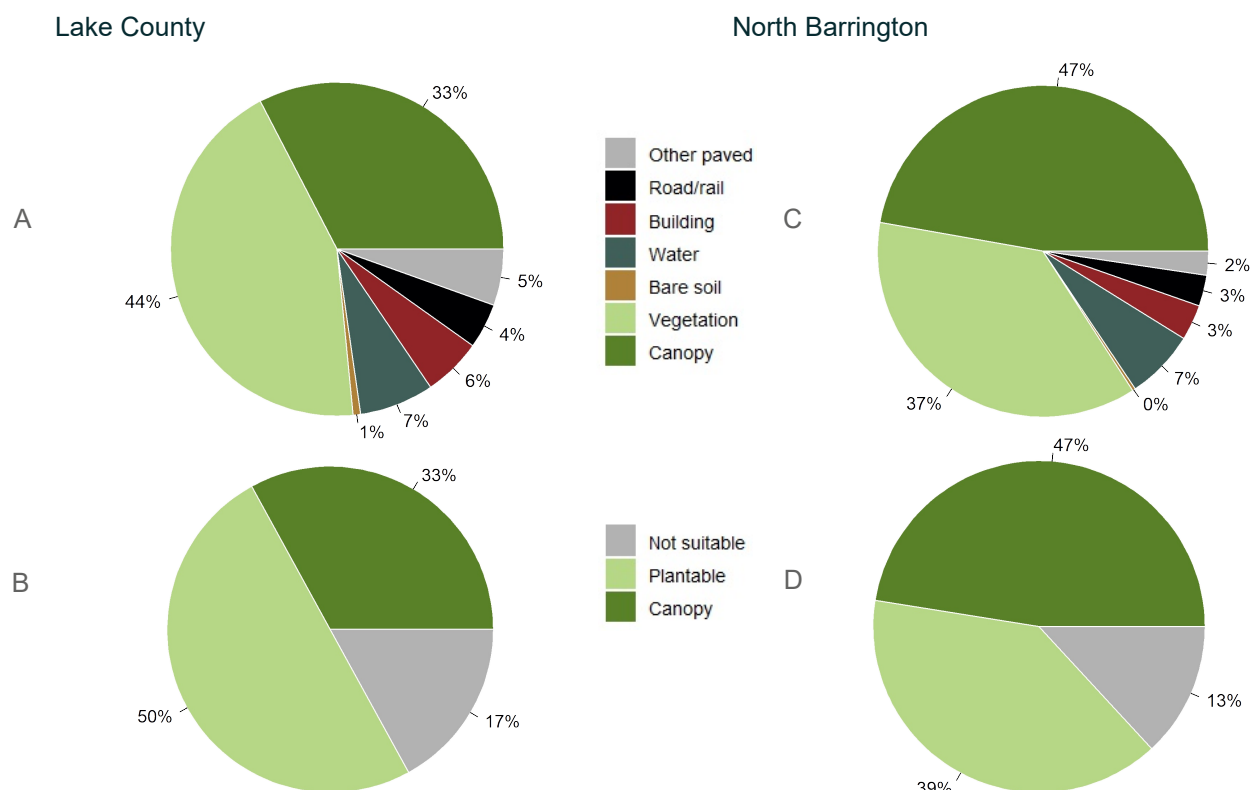
Figure 2: Land cover distribution and plantable space in Lake County (A and B) and in North Barrington (C and D).
