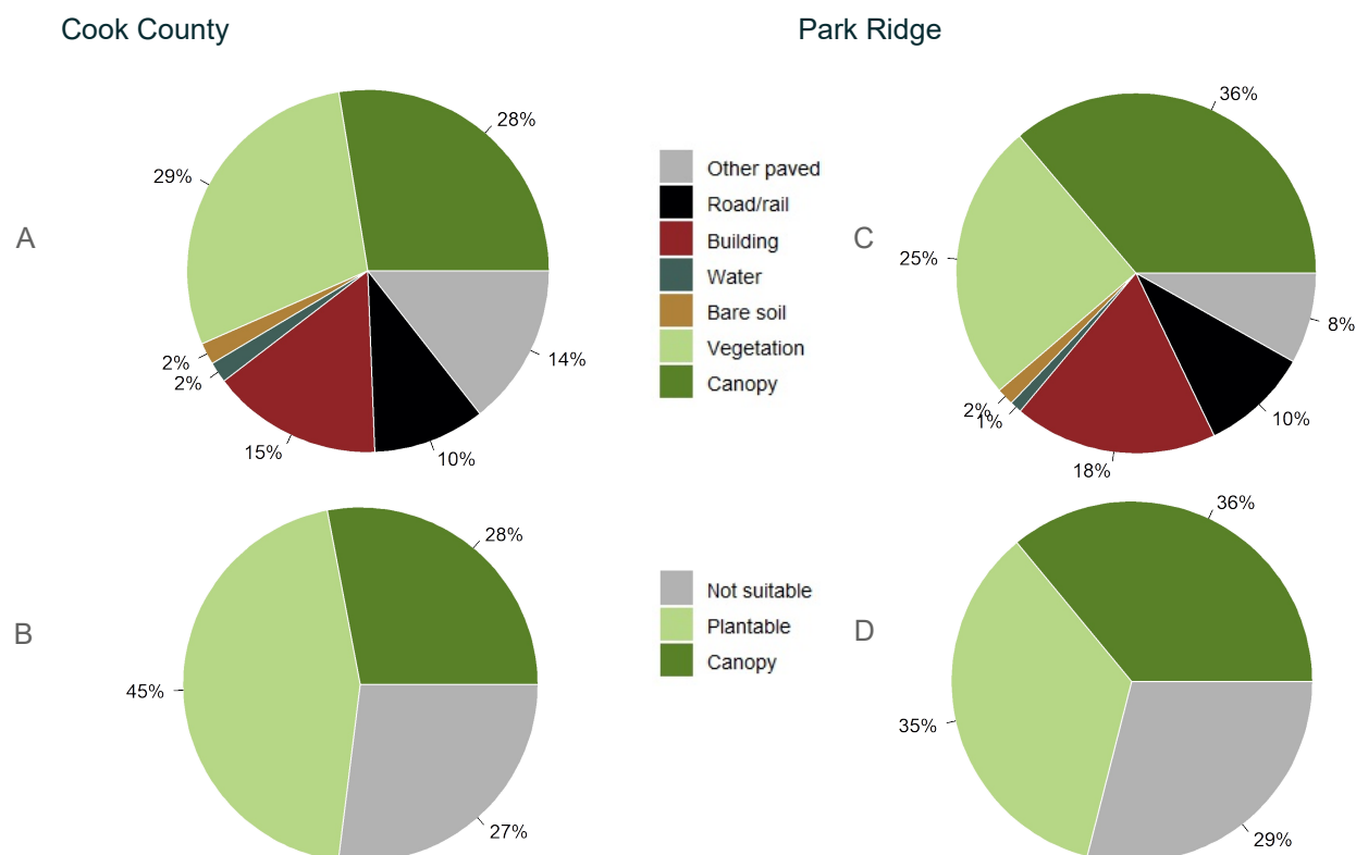
Figure 2: Land cover distribution and plantable space in Cook County (A and B), and in Park Ridge (C and D).
