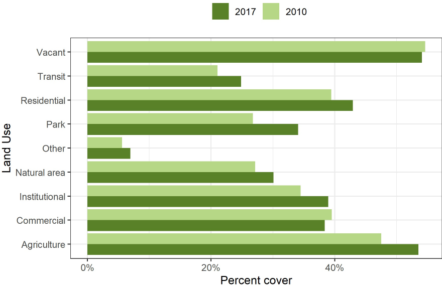
Figure 9: Canopy change across land use types in Port Barrington.
