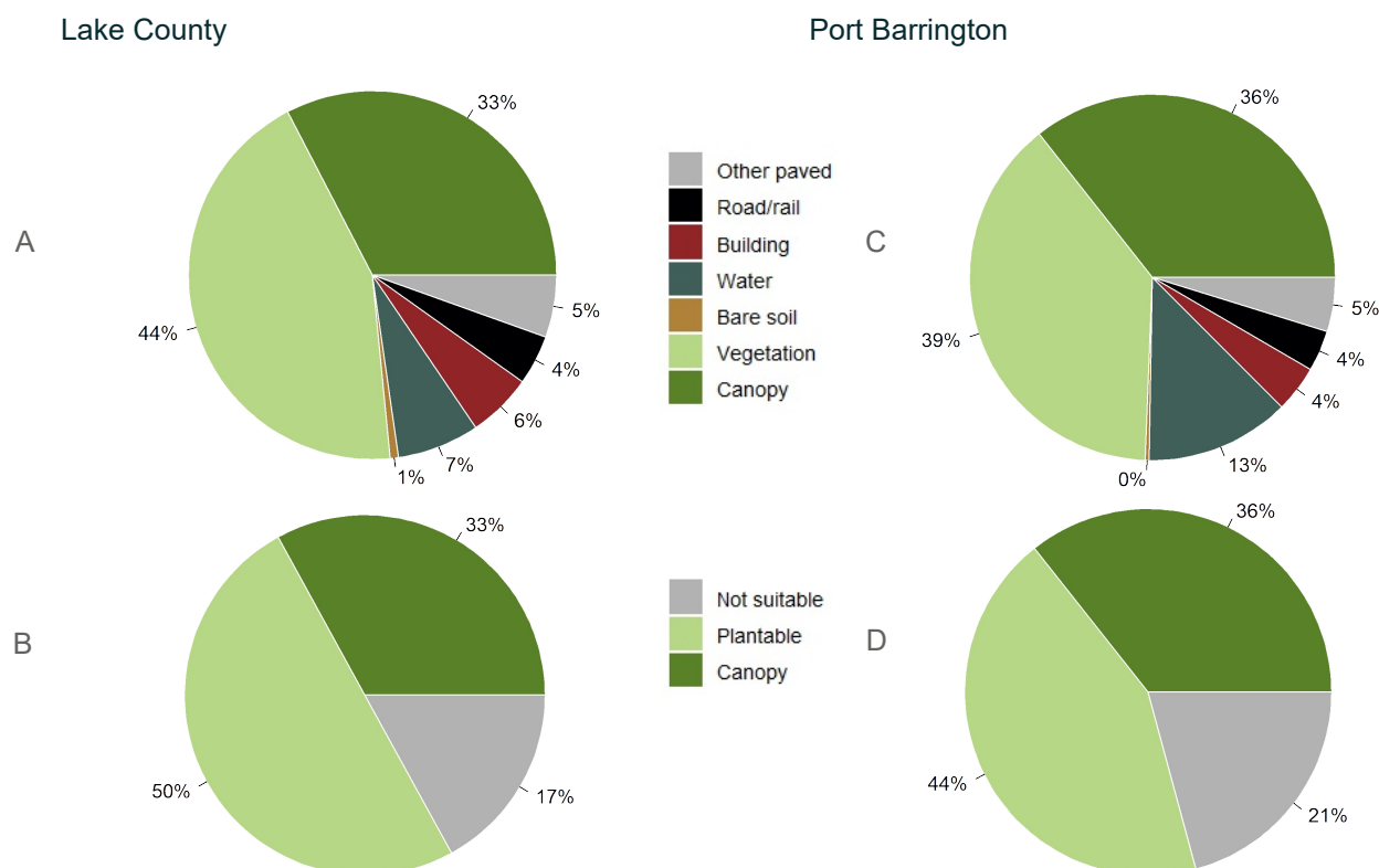
Figure 2: Land cover distribution and plantable space in Lake County (A and B) and in Port Barrington (C and D).
