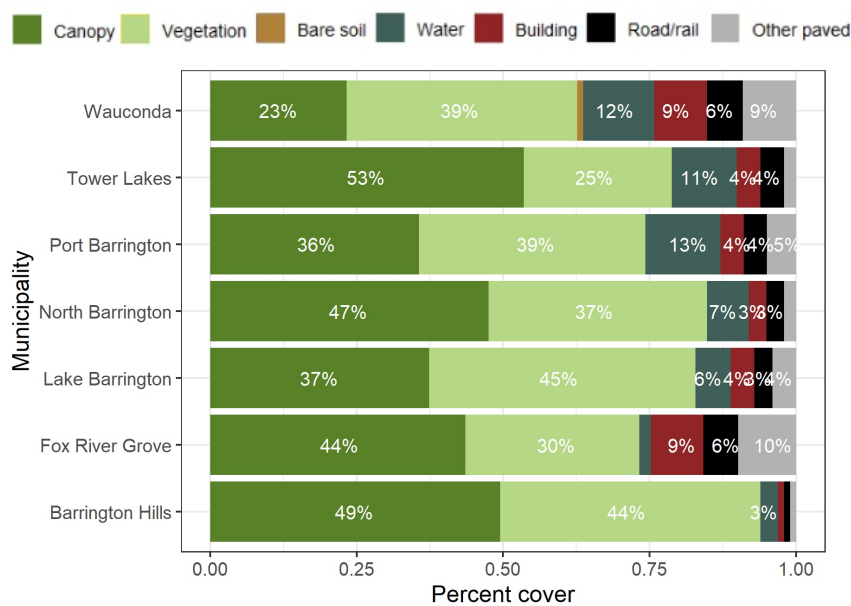
Figure 7: Comparison of land cover of Port Barrington and its neighbors.
