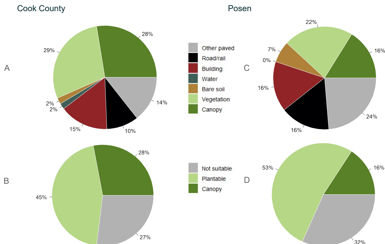
Figure 2: Land cover distribution and plantable space in Cook County (A and B) and in Posen (C and D).
