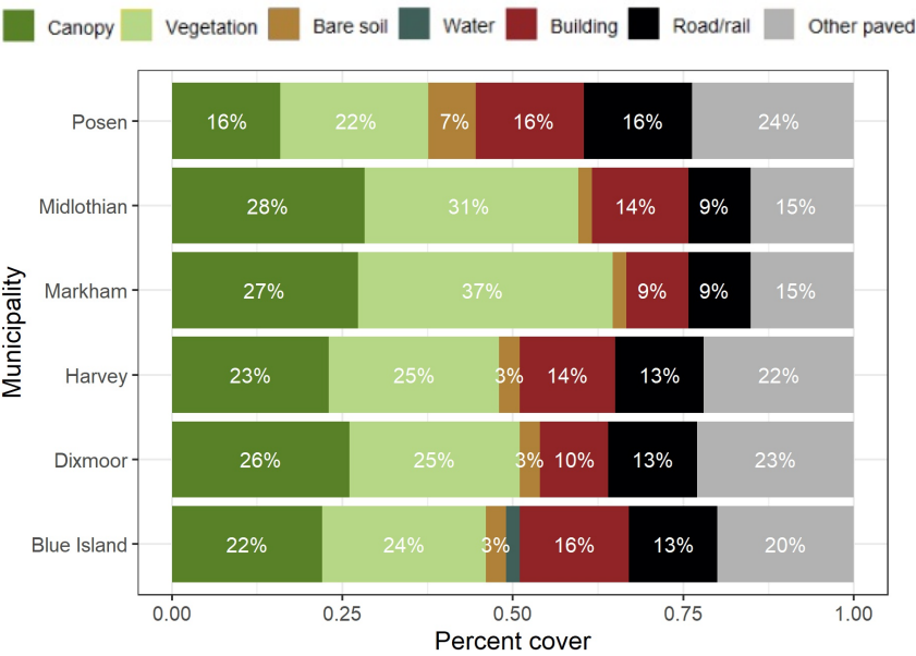
Figure 7: Comparison of land cover of Posen and its neighbors.
