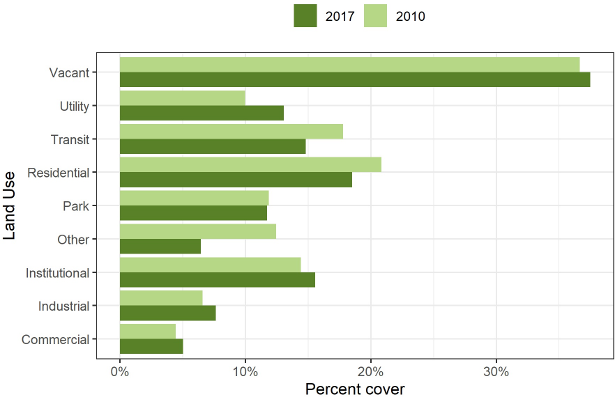
Figure 9: Canopy change across land use types in Posen.
