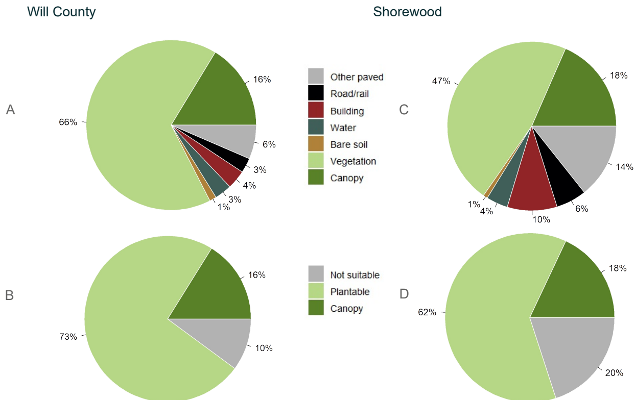
Figure 2: Land cover distribution and plantable space in Will County (A and B) and in Shorewood (C and D).
