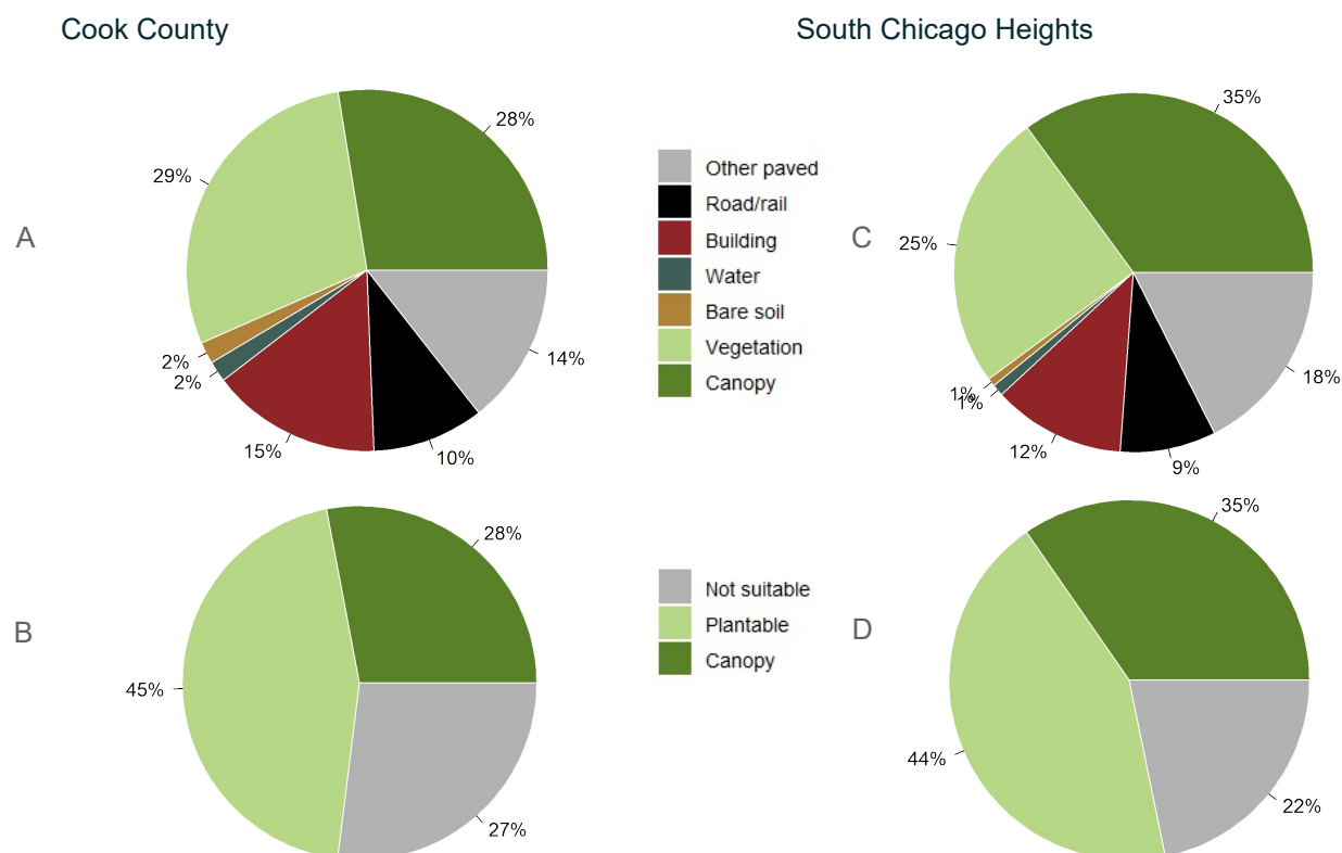
Figure 2: Land cover distribution and plantable space in Cook County (A and B) and in South Chicago Heights (C and D).
