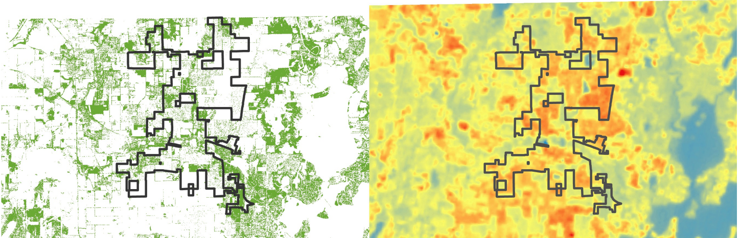
Figure 13: The image on the left shows tree canopy and on the right shows surface temperature. Surface temperature was calculated using a LandSat8 image from July 2017. Areas that have higher tree canopy tend to have lower temperatures.
