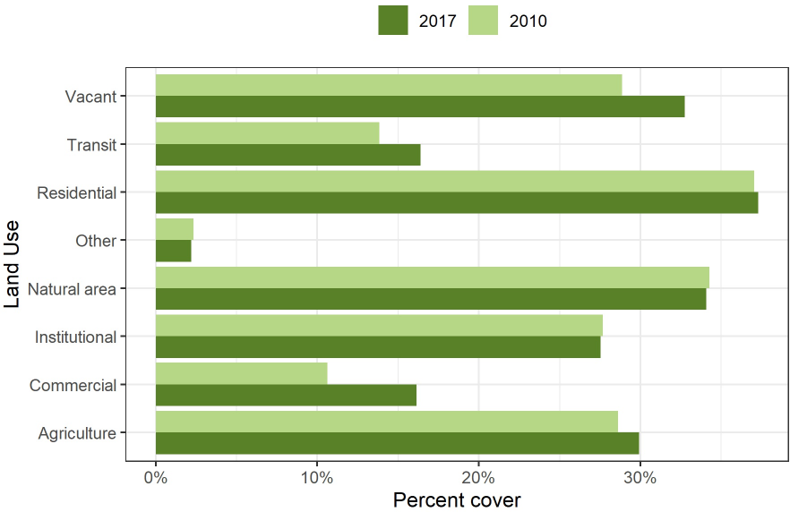
Figure 9: Canopy change across land use types in Third Lake.
