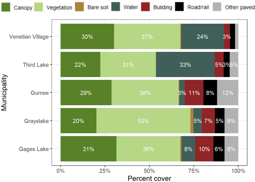
Figure 7: Comparison of land cover of Third Lake and its neighbors.
