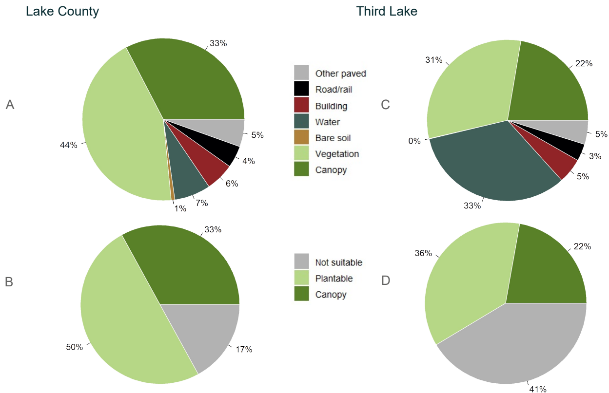
Figure 2: Land cover distribution and plantable space in Lake County (A and B) and in Third Lake (C and D).
