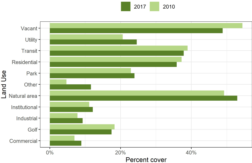
Figure 9: Canopy change across land use types in Villa Park.
