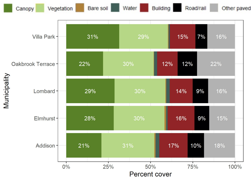
Figure 7: Comparison of land cover of Villa Park and its neighbors.
