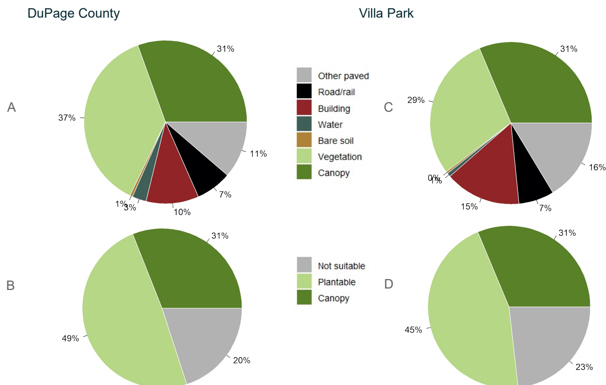
Figure 2: Land cover distribution and plantable space in DuPage County (A and B) and in Villa Park (C and D).
