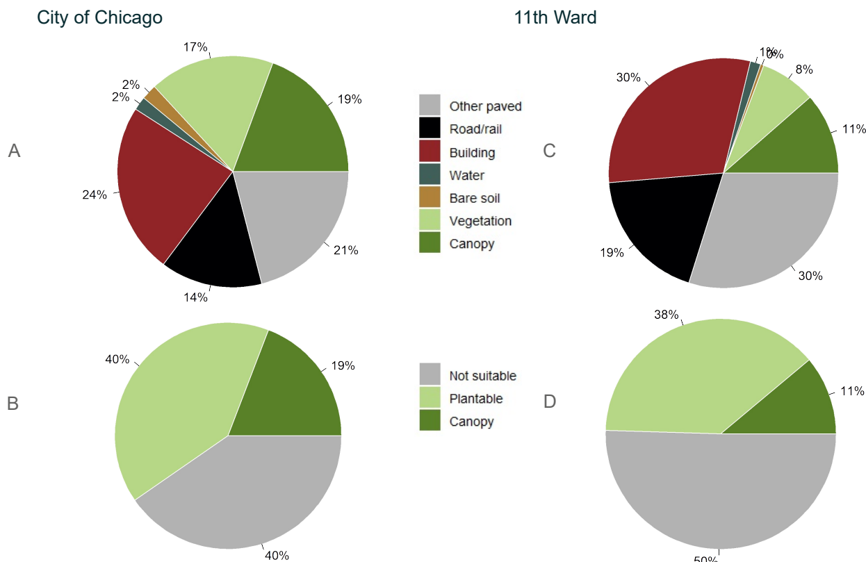
Figure 2: Land cover distribution and plantable space in the City of Chicago (A and B) and in the 11th Ward (C and D).
