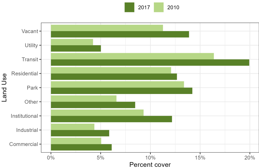
Figure 9: Canopy change across land use types in the 25th Ward.
