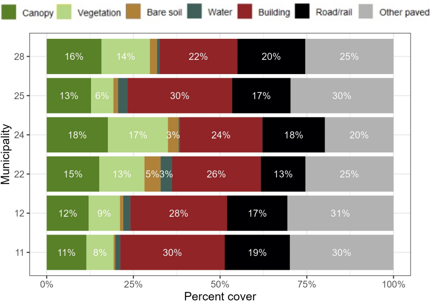
Figure 7: Comparison of land cover of the 25th Ward and its neighbors.
