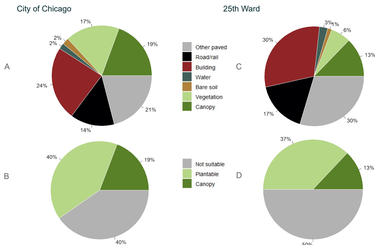
Figure 2: Land cover distribution and plantable space in the City of Chicago (A and B) and in the 25th Ward (C and D).
