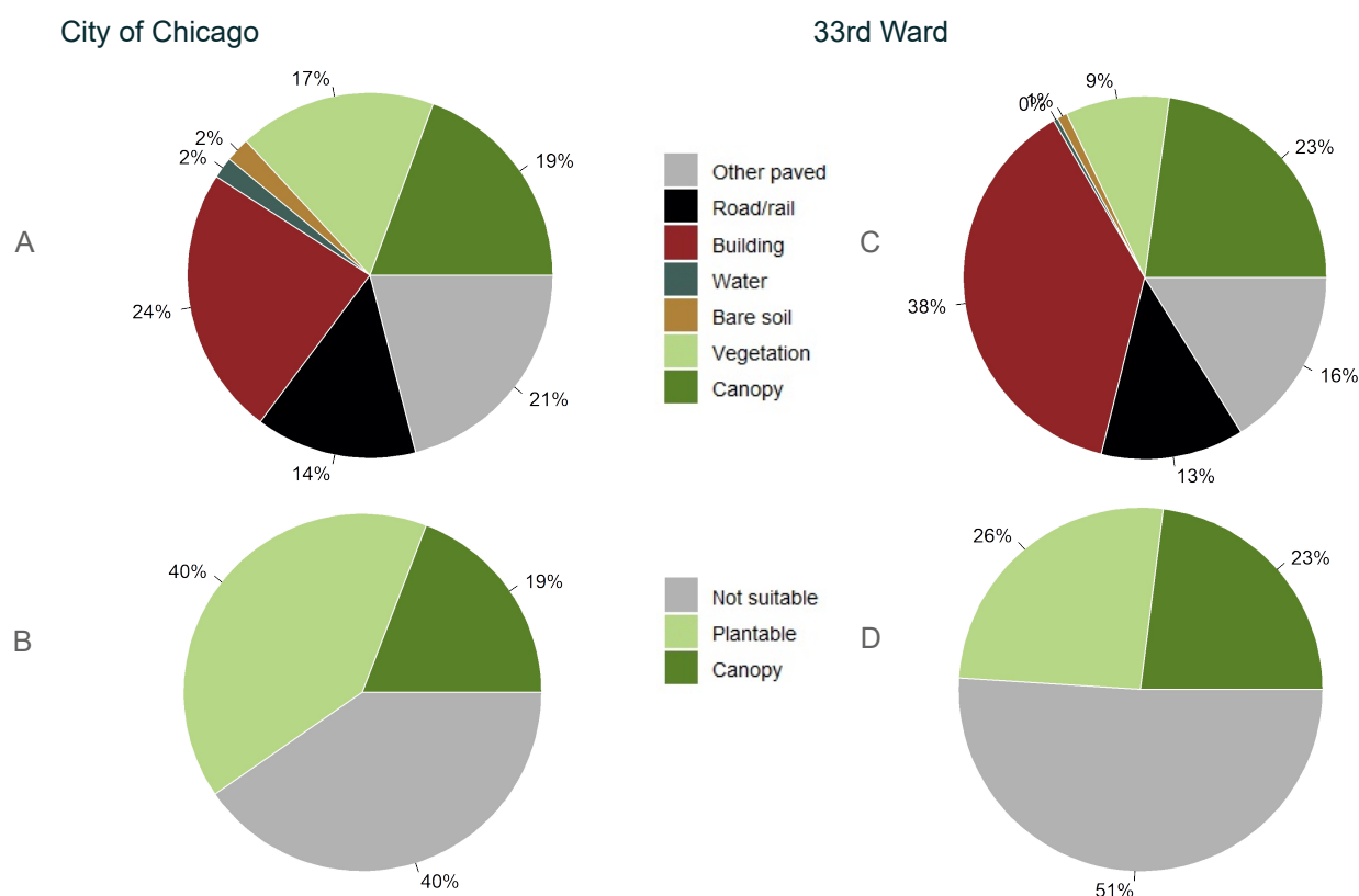
Figure 2: Land cover distribution and plantable space in the City of Chicago (A and B) and in the 33rd Ward (C and D).
