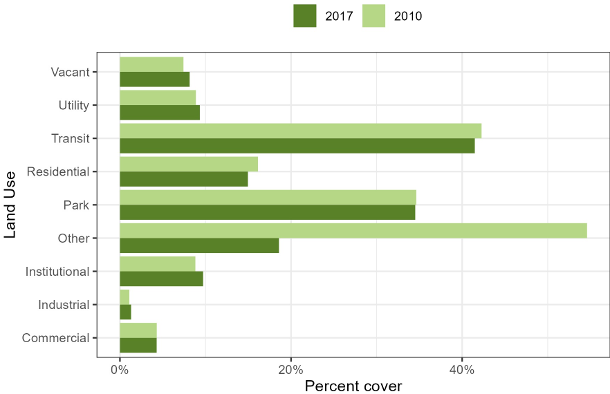
Figure 9: Canopy change across land use types in the 33rd Ward.
