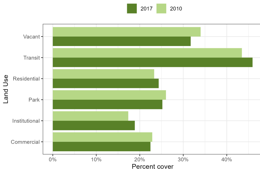
Figure 9: Canopy change across land use types in the 43rd Ward.
