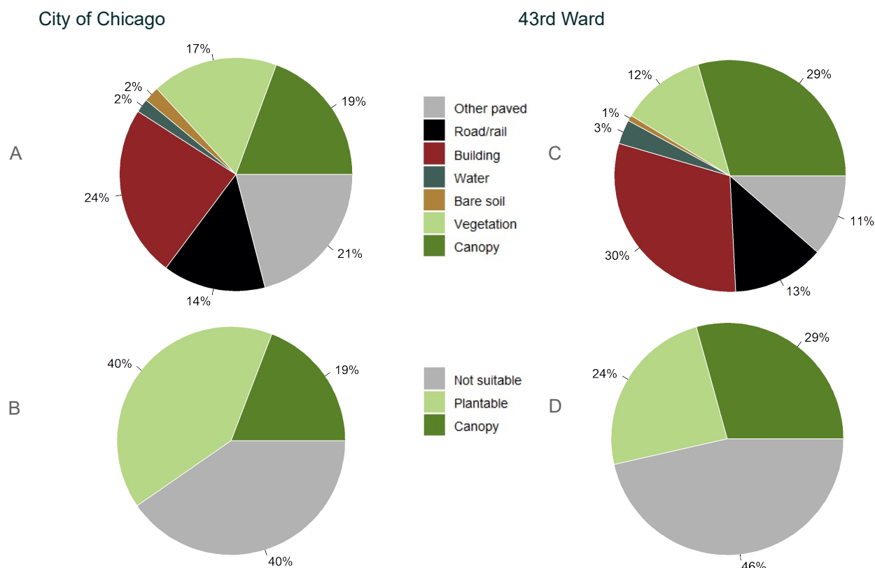
Figure 2: Land cover distribution and plantable space in the City of Chicago (A and B) and in the 43rd Ward (C and D).
