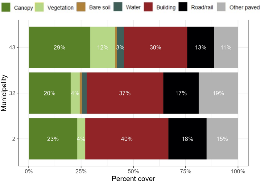
Figure 7: Comparison of land cover of the 43rd Ward and its neighbors.
