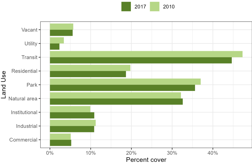
Figure 9: Canopy change across land use types in the 50th Ward.
