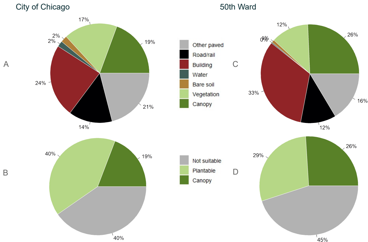
Figure 2: Land cover distribution and plantable space in the City of Chicago (A and B) and in the 50th Ward (C and D).
