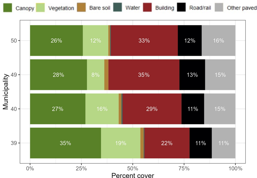
Figure 7: Comparison of land cover of the 50th Ward and its neighbors.
