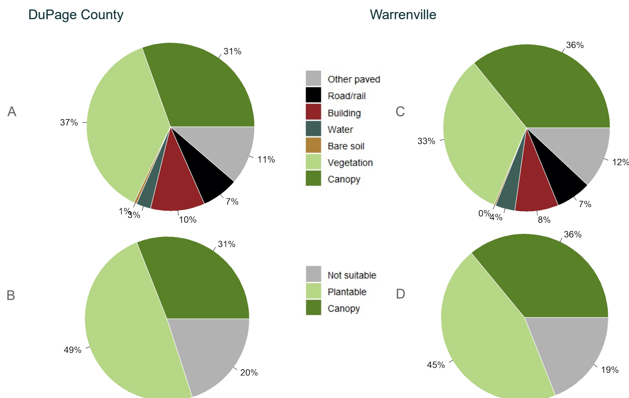
Figure 2: Land cover distribution and plantable space in DuPage County (A and B), and in Warrenville (C and D).
