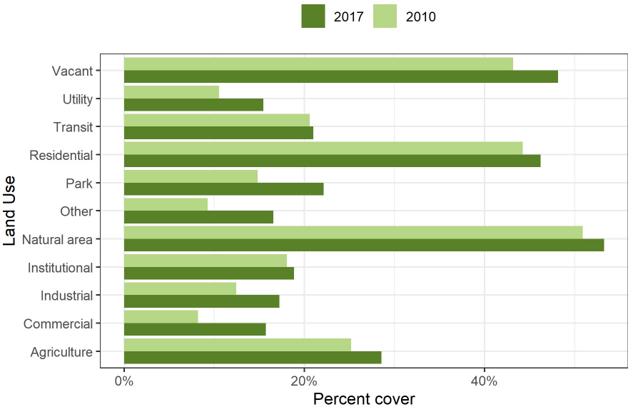
Figure 9: Canopy change across land use types in Warrenville.
