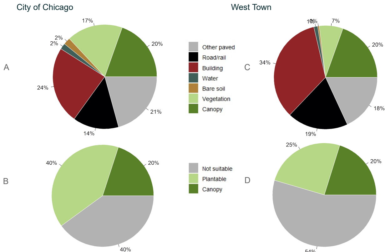
Figure 2: Land cover distribution and plantable space in the City of Chicago (A and B) and in West Town (C and D).
