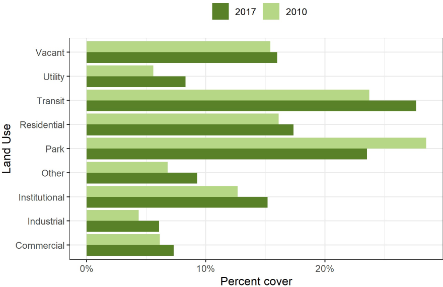
Figure 9: Canopy change across land use types in West Town.
