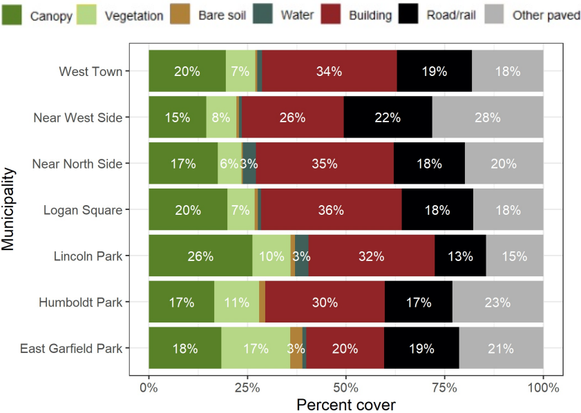
Figure 7: Comparison of land cover of West Town and its neighbors.
