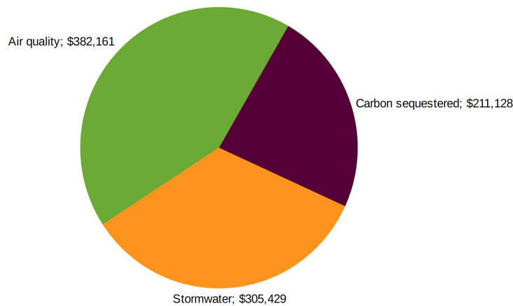
Figure 14: Trees offer myriad benefits, including intercepting stormwater, improving air quality and removing carbon from the atmosphere.
