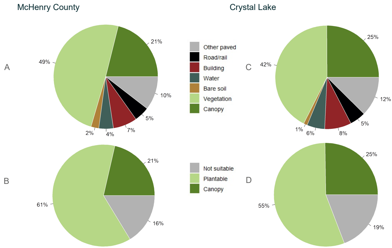
Figure 2: Land cover distribution and plantable space in McHenry County (A and B), and in Crystal Lake (C and D).
