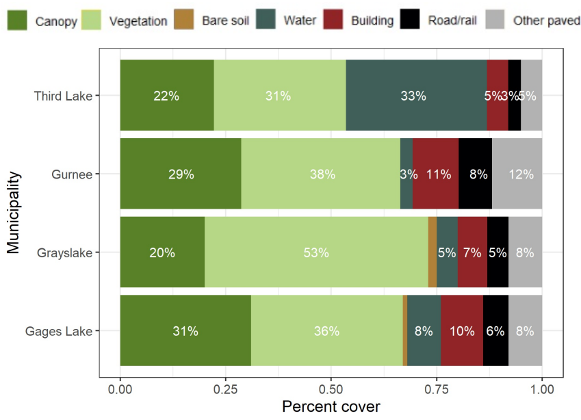
Figure 7: Comparison of land cover of Gages Lake and its neighbors.
