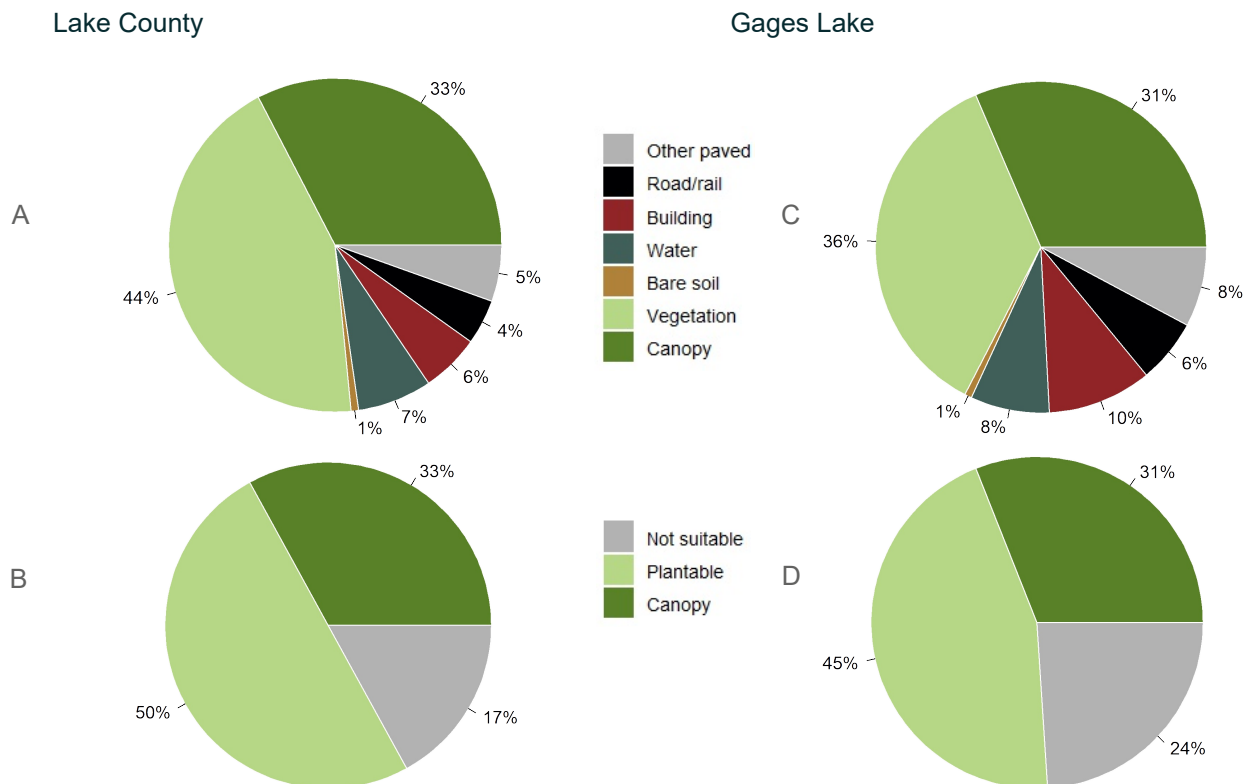
Figure 2: Land cover distribution and plantable space in Lake County (A and B), and in Gages Lake (C and D).
