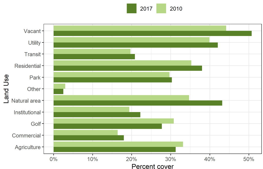
Figure 9: Canopy change across land use types in Gages Lake.
