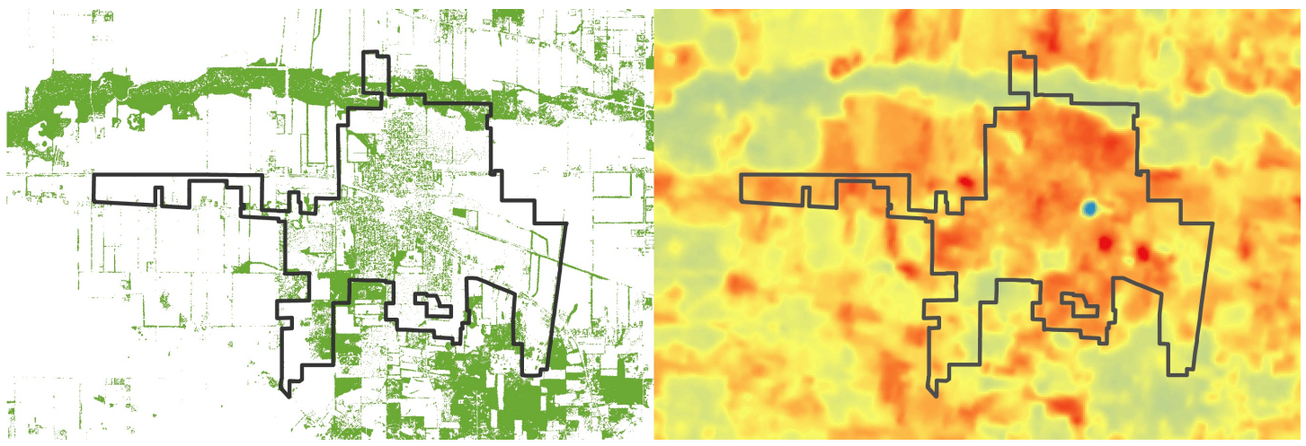
Figure 13: The image on the left shows tree canopy and on the right shows surface temperature. Surface temperature was calculated using a LandSat8 image from July 2017. Areas that have higher tree canopy tend to have lower temperatures.
