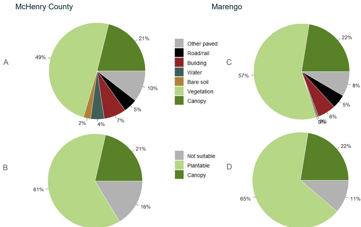
Figure 2: Land cover distribution and plantable space in McHenry County (A and B), and in Marengo (C and D).
